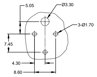
RECOMMENDED LAYOUT VIEW FROM COMPONENTS SIDE OF PCB
