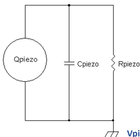
Figure 3(a) - Charge model of piezo device
