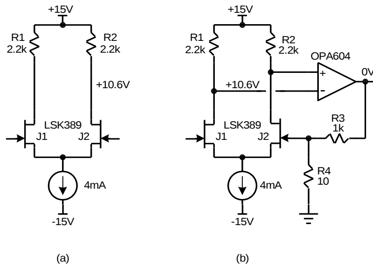
Figure 4: Simple LSK389 differential amplifiers
