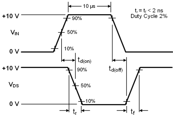
TIMING WAVEFORMS
