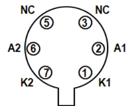
ID101 TO-71 TOP VIEW
