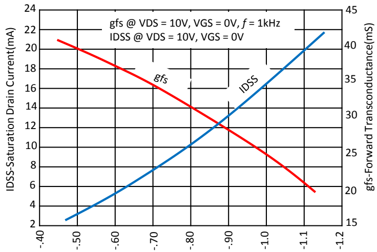
Drain Current Transconductance vs. Gate-Source Cutoff Voltage
