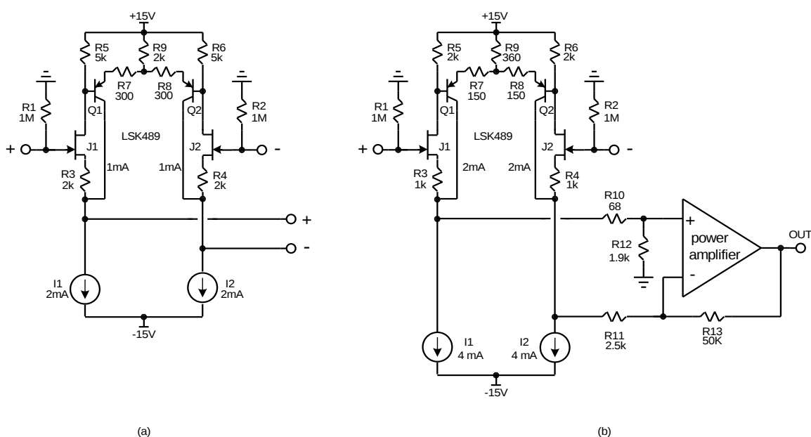
Figure 4: Differential CFP FET Buffer
