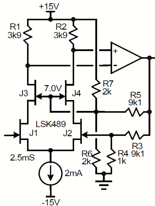
Figure 4: Driven Cascode FET Pair
