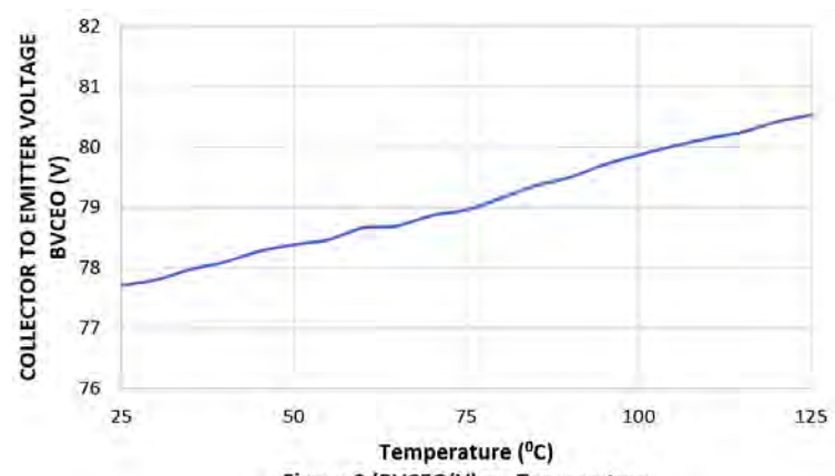
Figure-3 BVCEO(V) vs. Temperature
