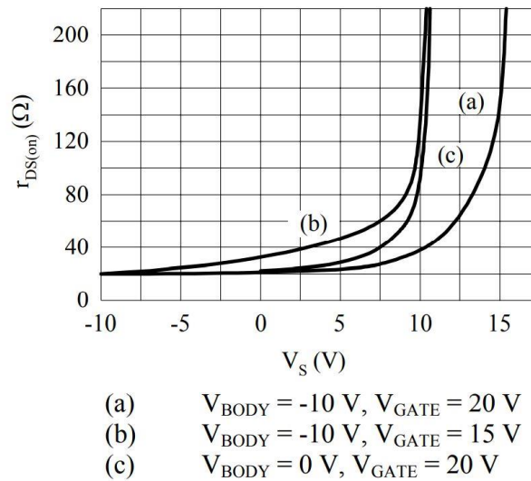
Figure 5. On Resistance Characteristics
