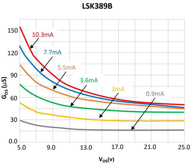
Figure 6. Output Conductance - G_{OS} vs. V_{DS} vs. I_D
