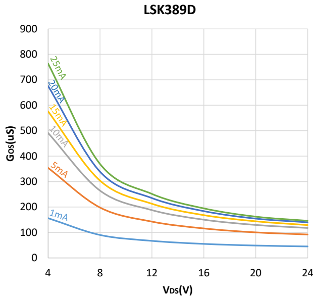
Figure 8. Output Conductance - G_{OS} vs. V_{DS} vs. I_D
