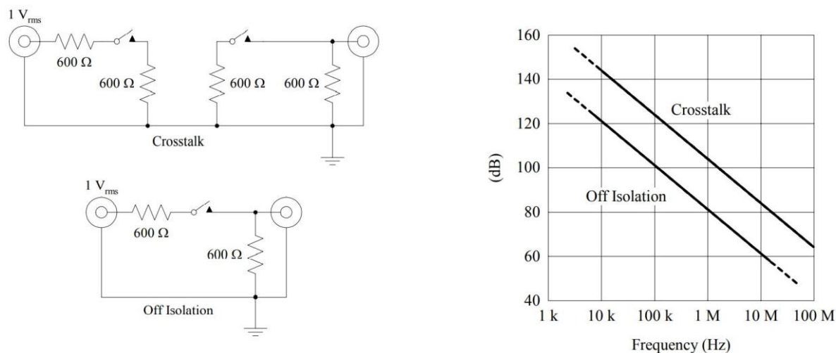
Figure 11. SD5000 Crosstalk and Off Isolation vs Frequency
