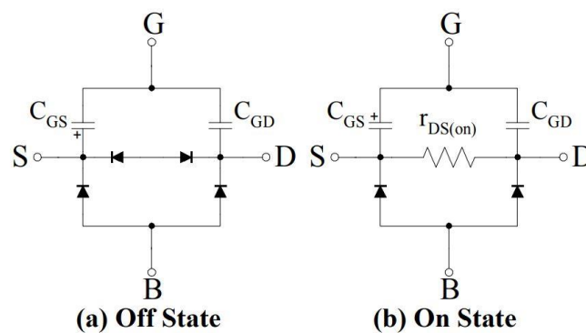
Figure 3. Equivalent Circuits
