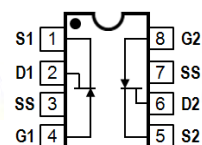
PDIP 8L Top View
