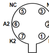
ID100 TO-78 TOP VIEW
