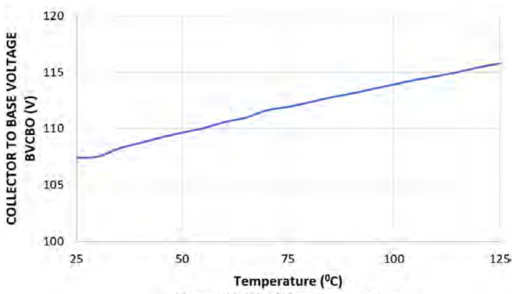
Figure-2 VBCBO(V) vs. Temperature
