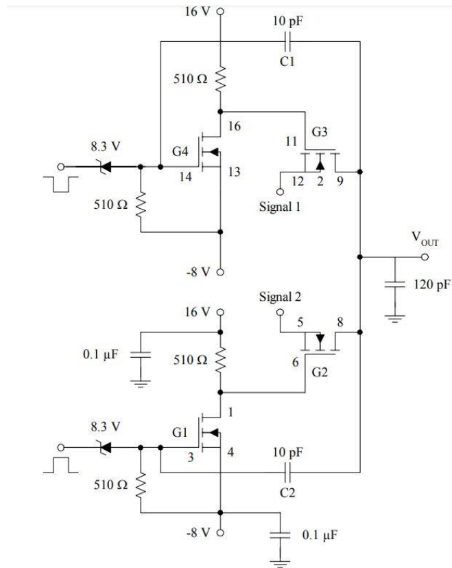
Figure 14. 5-MHz Multiplexer and Sample and Hold Circuit
