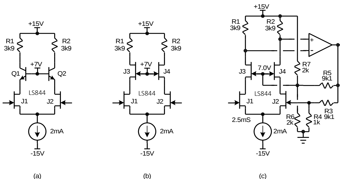
Figure 6: JFET Cascodes
