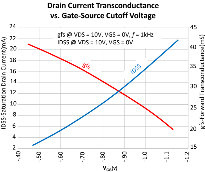
Figure 21. V GS (cutoff) vs. I DSS vs. G FS
