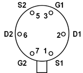
TO-71 & TO-78 TOP VIEW
