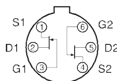
U SERIES TO-71 TOP VIEW
