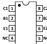
PDIP 8L Top View
