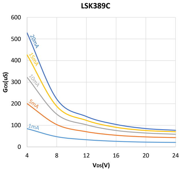
Figure 7. Output Conductance - G_{OS} vs. V_{DS} vs. I_D
