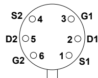
TO-71 6L Top View
