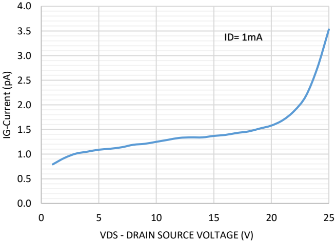
Operating Gate Current
