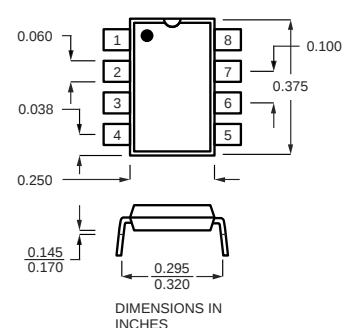
PDIP 8L
