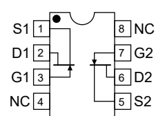
SST SERIES SOIC TOP VIEW
