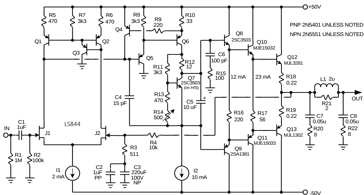
Figure 11: Power Amplifier
