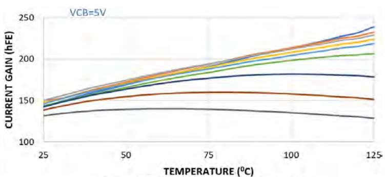
Figure-6 CURRENT GAIN (hFE) vs. Temperature
