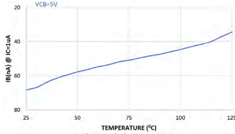
Figure-4 IB(nA) vs. Temperature
