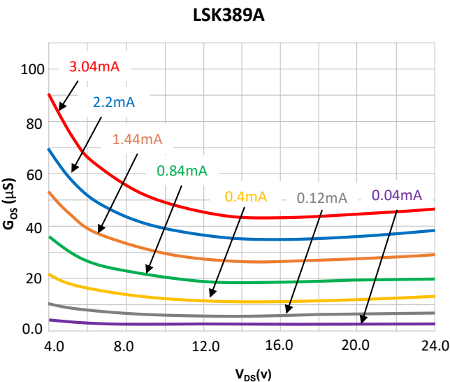
Figure 5. Output Conductance - G_{OS} vs. V_{DS} vs. I_D
