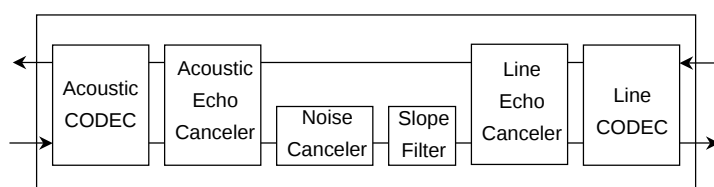
Figure 6 Dual Echo Canceler Mode
