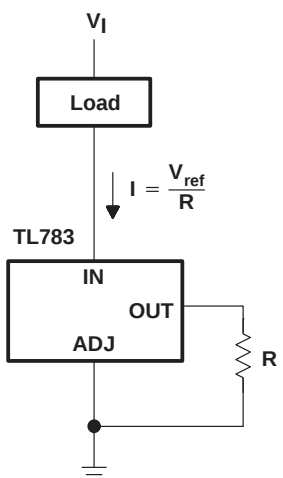
Figure 21. Current-Sinking Regulator
