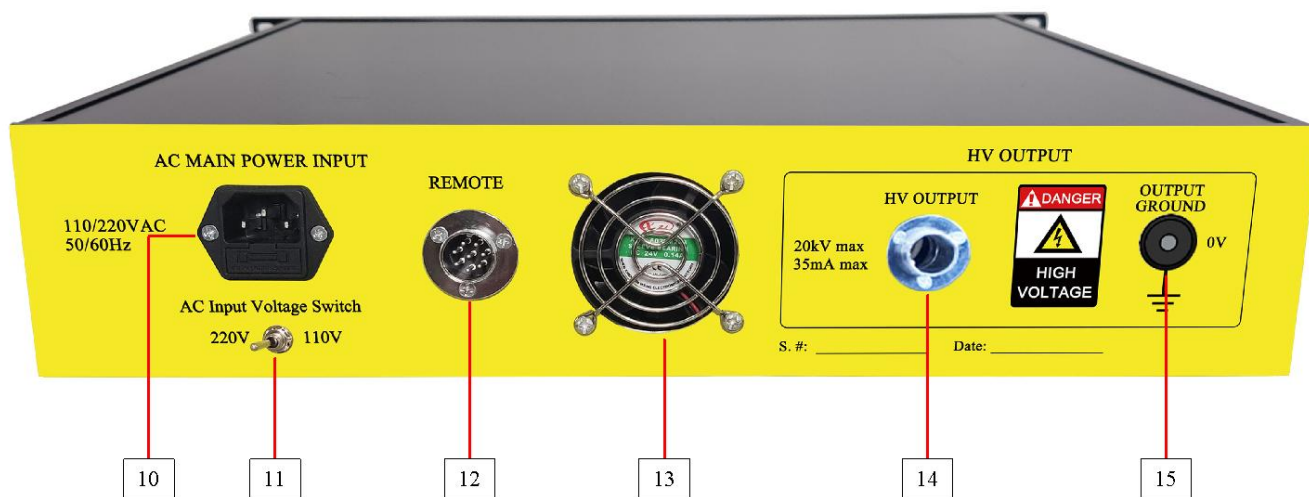
Figure 3. Front Panel
