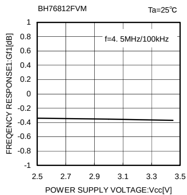
Fig. 25 Frequency response 1 vs. Supply voltage
