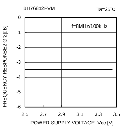
Fig. 27 Frequency response 2 vs. Supply voltage
