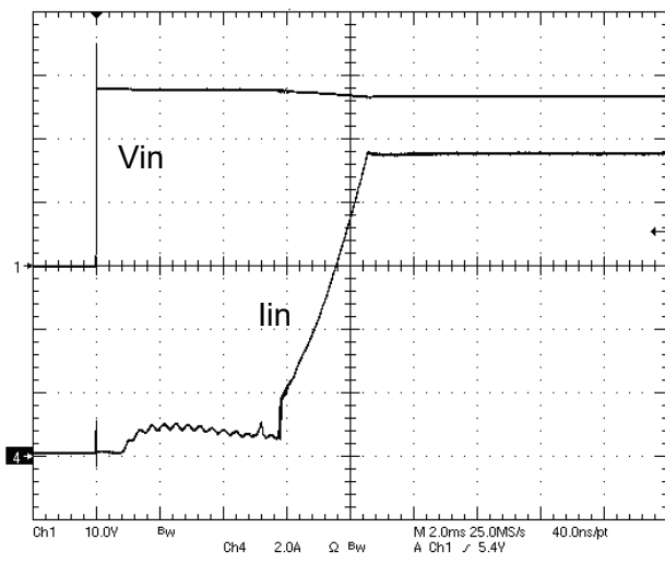
Figure 4 – Vin, lin during turn-on at 28V with DVME28, Cout=100 \mu F and 2x DVFL2800S at full load
