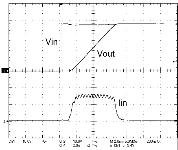
Figure 6 – Vin, Vout, lin during turn-on at 28V, Cout=500 \mu F
