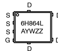
DFN5 (SO-8FL) CASE 488AA STYLE 1
