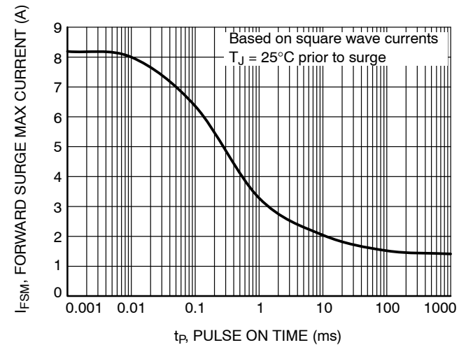
Figure 10. Forward Surge Current
