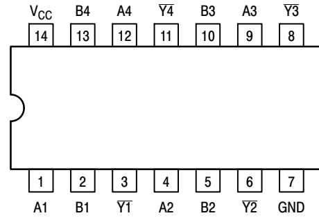
Figure 2. Pinout (Top View)
