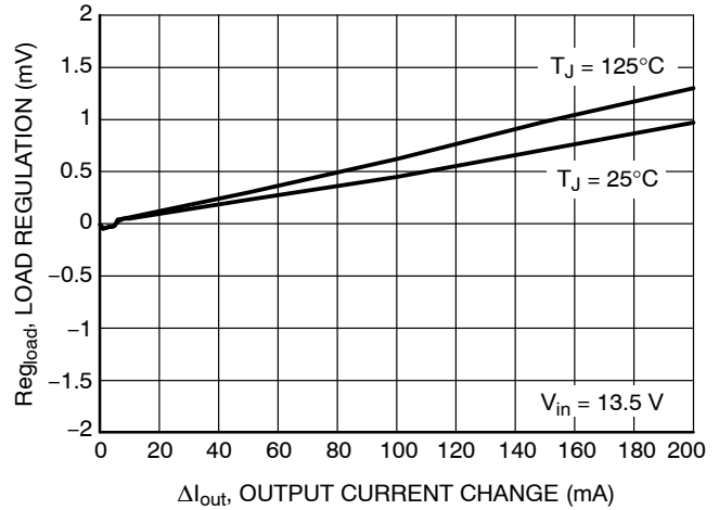
Figure 11. Load Regulation vs. Output Current Change
