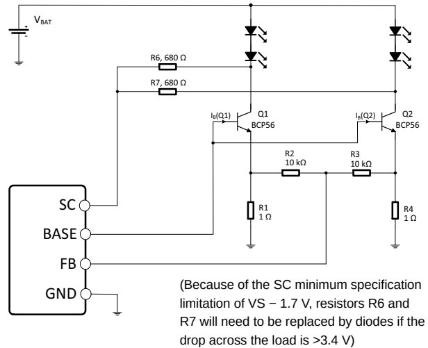
Figure 17. Driving Multiple Strings
