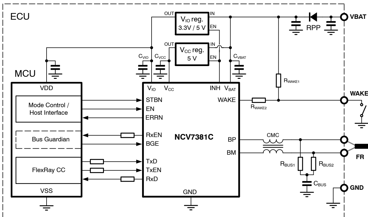
Figure 2. Application Diagram
