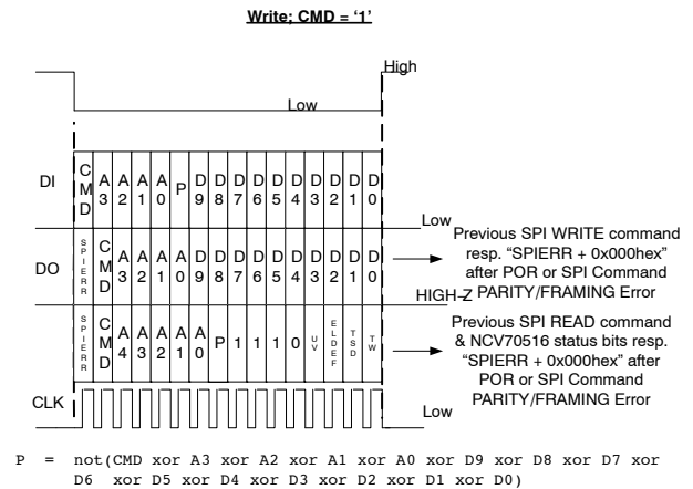
Figure 18. SPI Write Frame
