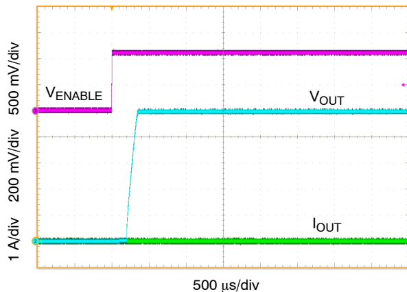
Figure 13. Enable Transient Response, I_{OUT} = 0\text{ A} , C_{OUT} = 10\text{ µF MLCC} , C_{SS} = 0\text{ nF}
