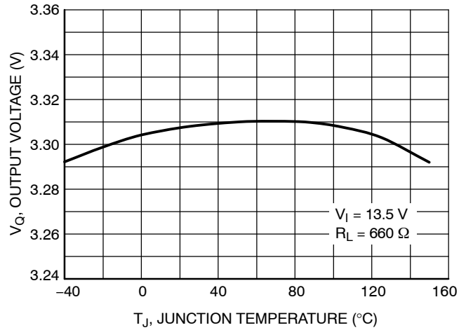
Figure 13. Output Voltage vs. Junction Temperature
