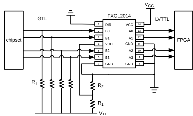
Figure 8. Application Diagram for GTL to LVTTL
