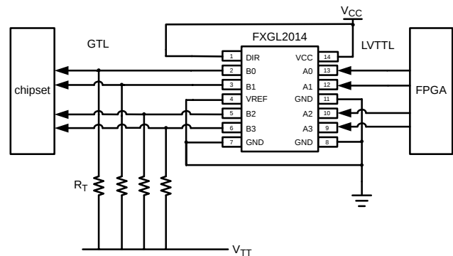
Figure 9. Application Diagram for LVTTL to GTL
