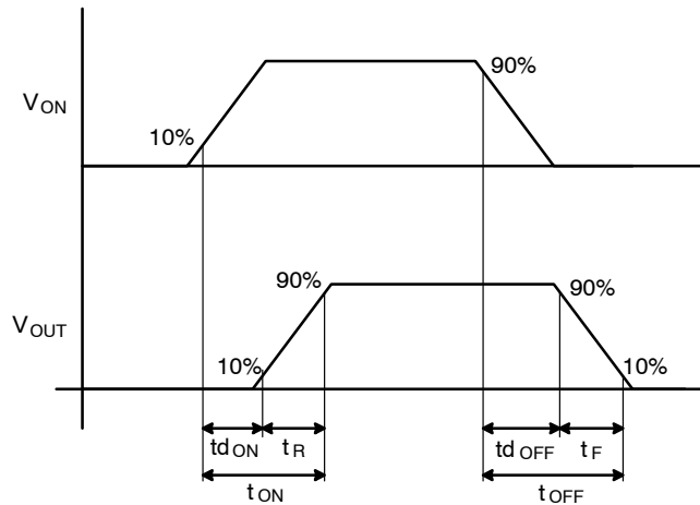
Figure 5. Timing Diagram
