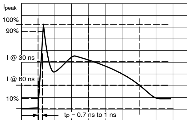
Figure 11. IEC61000-4-2 Spec
