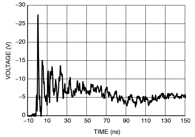
Figure 8. Negative 8 kV ESD Contact Discharge
