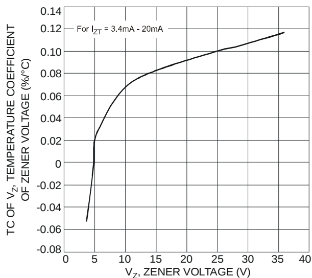
Fig. 6 Typical Temperature Coefficient of Zener Voltage vs. Zener Voltage (MMSZ5227B - MMSZ5258B)
