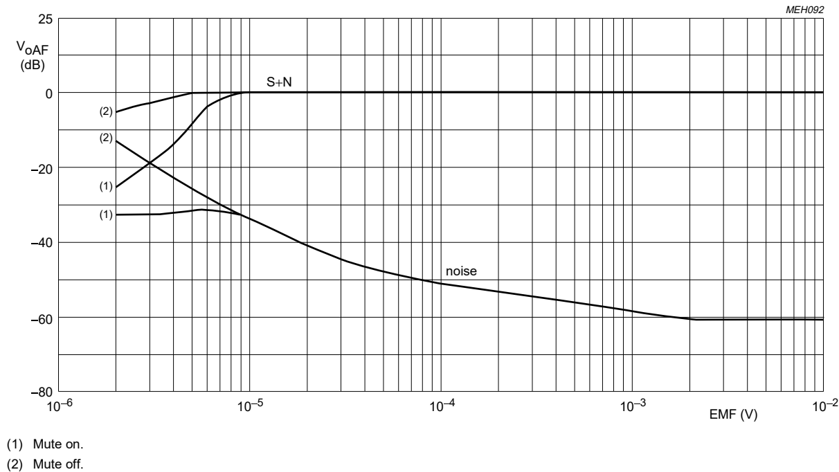
Fig.3 Input sensitivity.
