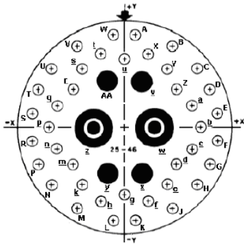
Contact Layout
