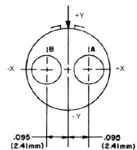
Contact Layout
