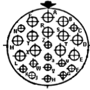
Contact Layout
