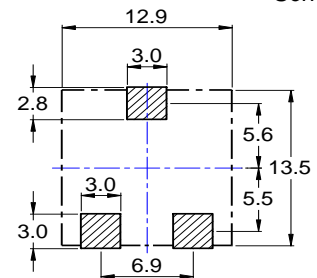
Reference Land Pattern
