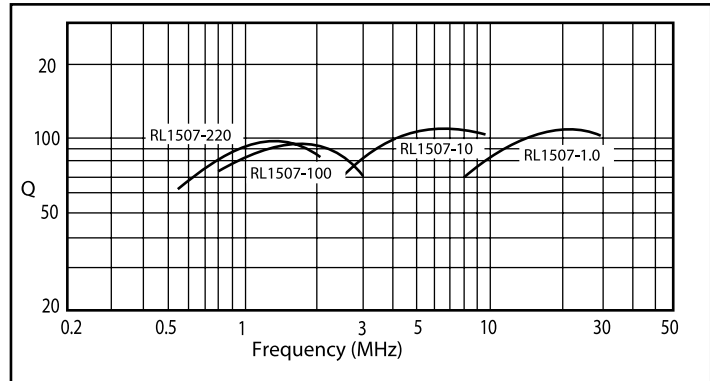
Q-Frequency Characteristics
