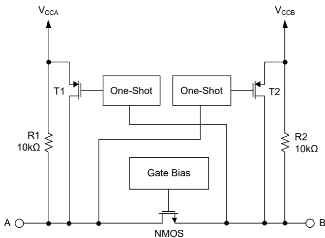
Figure 7. Architecture of an SGM4553 Cell
