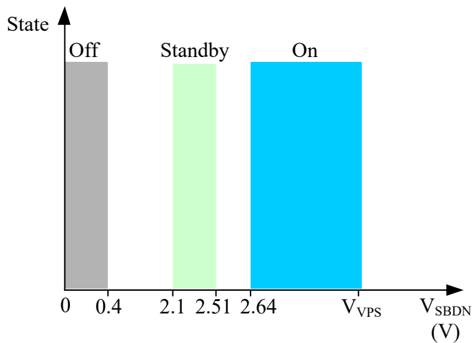
Figure 3. V_{\text{SBDN}} vs. Amplifier States
