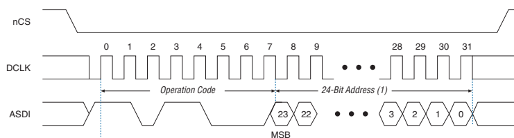
Figure 4-16. Erase Sector Operation Timing Diagram
