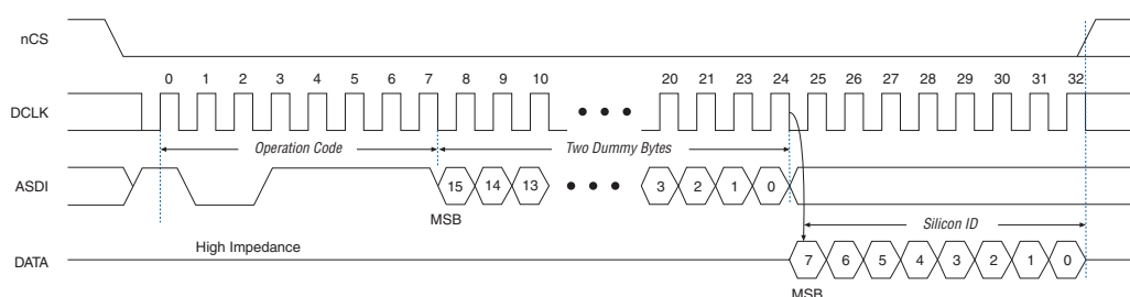
Figure 4-13. Read Device Identification Operation Timing Diagram (Note 1)
