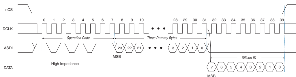
Figure 4-12. Read Silicon ID Operation Timing Diagram (Note 1)
