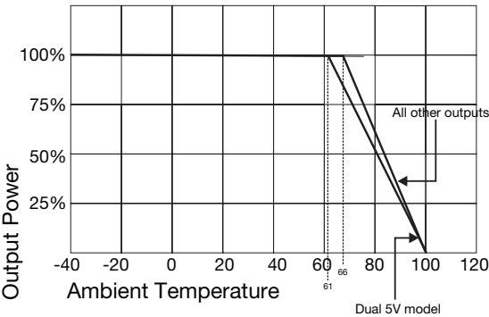
Without heatsink
