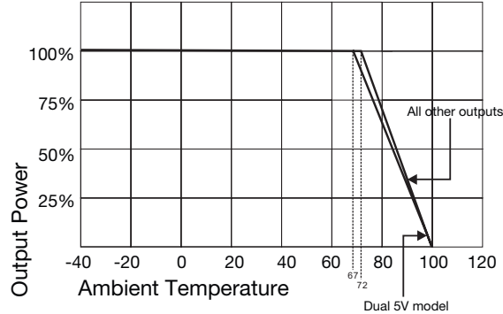
With heatsink
