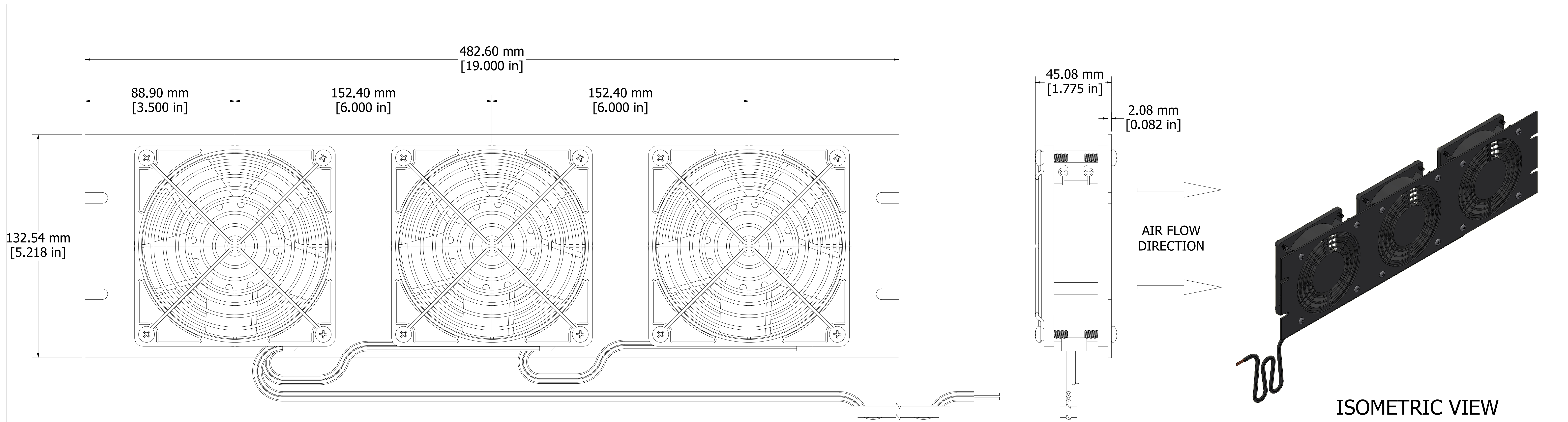
ASSEMBLY - VIEW FROM REAR
