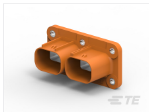
TE Part #2103346-1 HVA280 2 Bay Header Sub-Assy, KEY A, E
