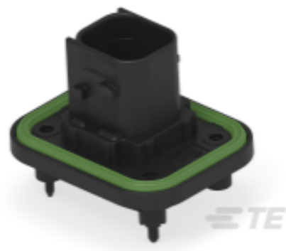
TE Part #1-2377473-1 4POS,TAB2.8X0.8,HDR ASSY,180DEG, COD A
