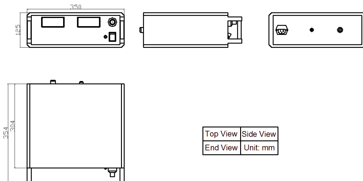
Figure 7. Dimensions for AHVACN40KVR5MABT
