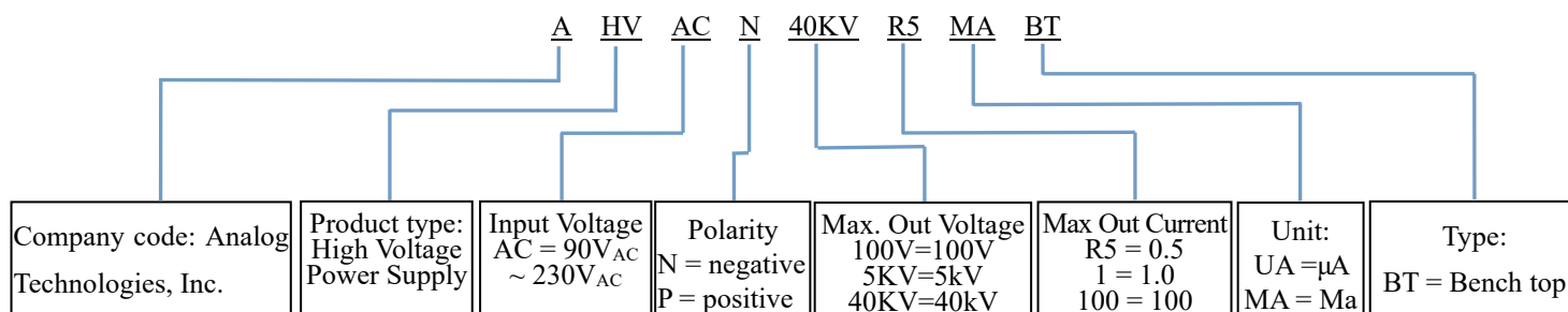
Figure 5. Naming Rules of AHVACN40KVR5MABT
