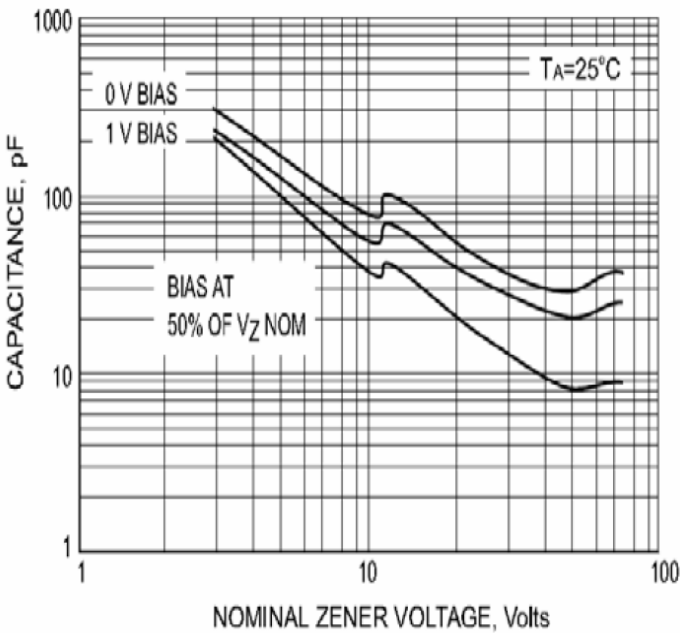
Fig.4 Typical Total Capacitance vs. Nominal Zener Voltage
