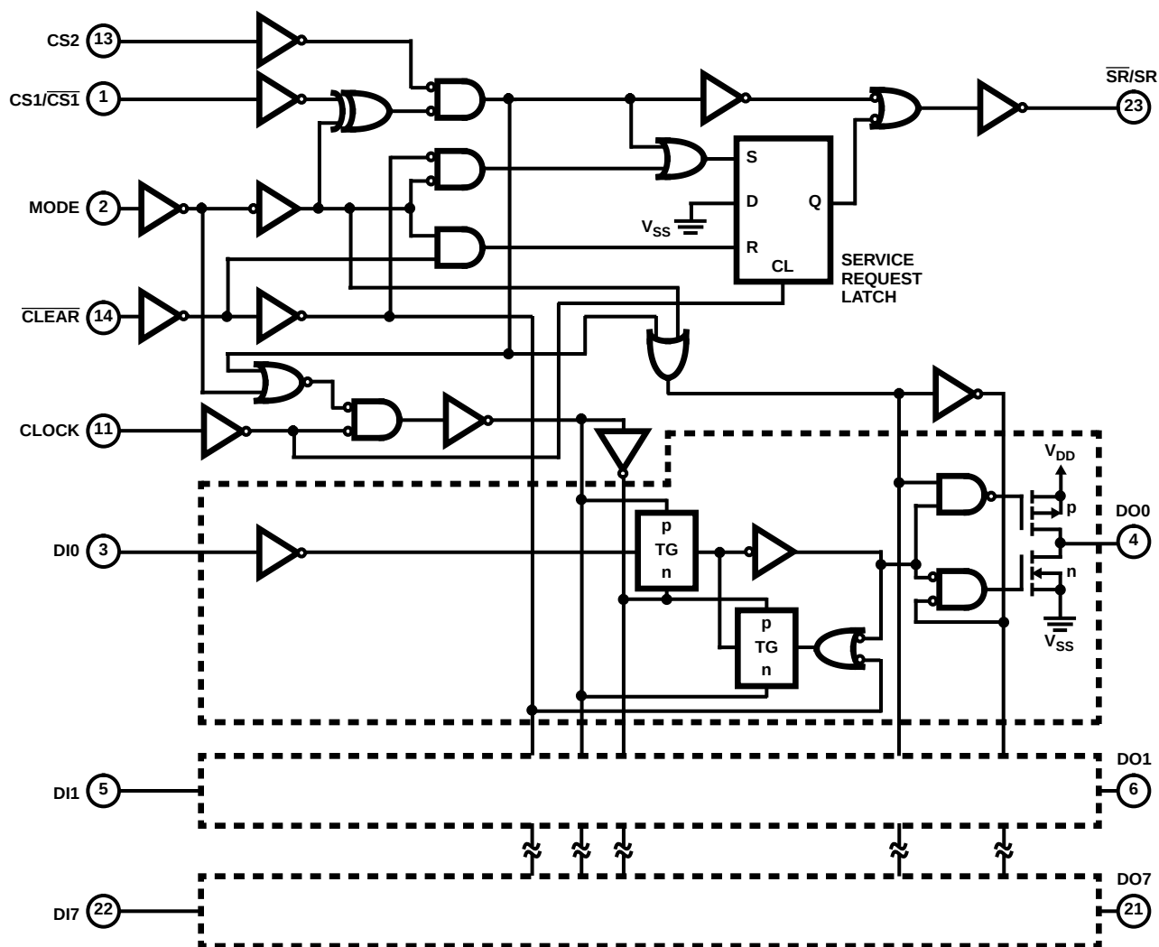
FIGURE 3. CDP1852 LOGIC DIAGRAM
