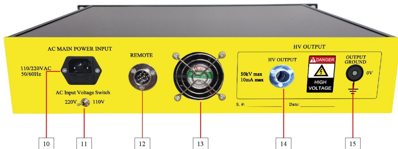
Figure 3. Front Panel
