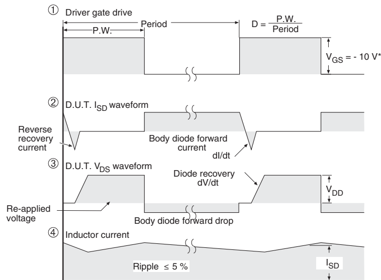
Fig. 14 - For P-Channel
