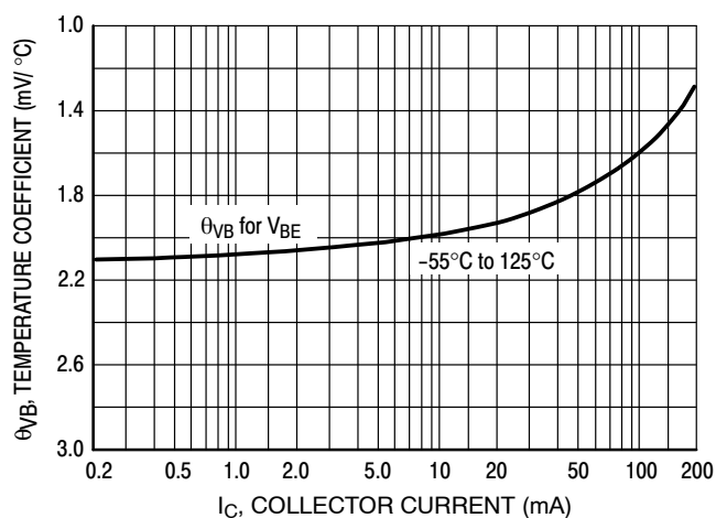
Figure 14. Base-Emitter Temperature Coefficient
