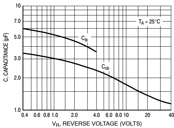
Figure 7. Capacitances
