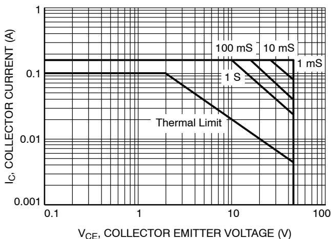
Figure 34. Safe Operating Area for LBC847A, LBC847B, LBC847C
