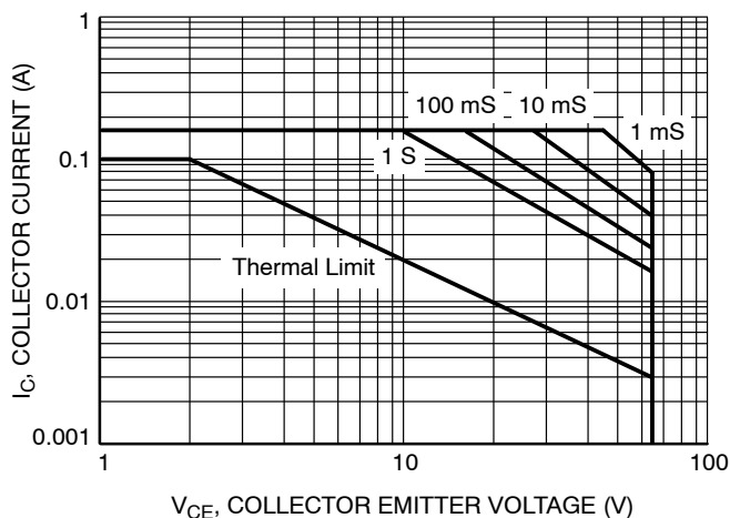
Figure 33. Safe Operating Area for LBC846A, LBC846B
