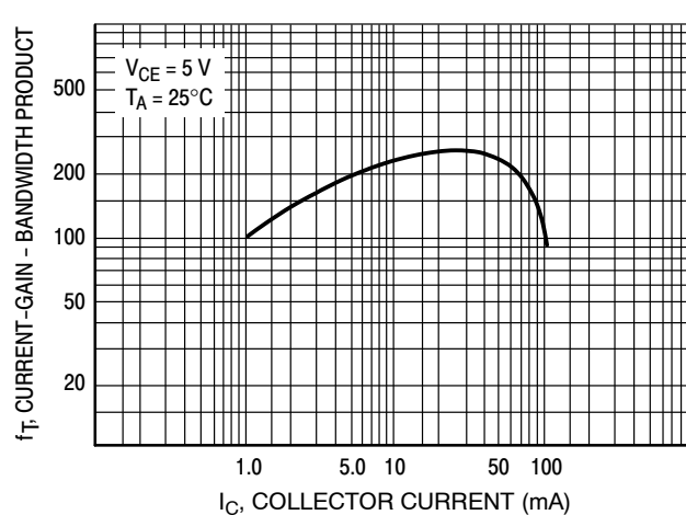
Figure 16. Current-Gain - Bandwidth Product
