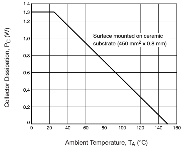
Figure 10. P_C - T_A
