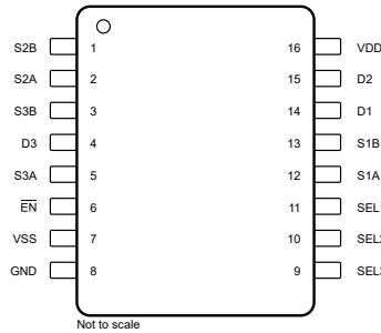
Figure 5-7. TMUX4053 PW Package, 16-Pin TSSOP (Top View)
