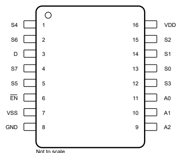
Figure 5-1. TMUX4051 PW Package, 16-Pin TSSOP (Top View)
