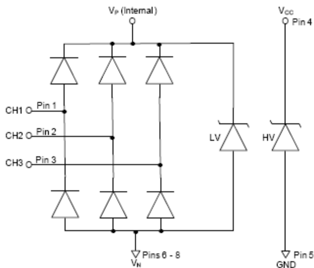
Figure 1. Electrical Schematic
