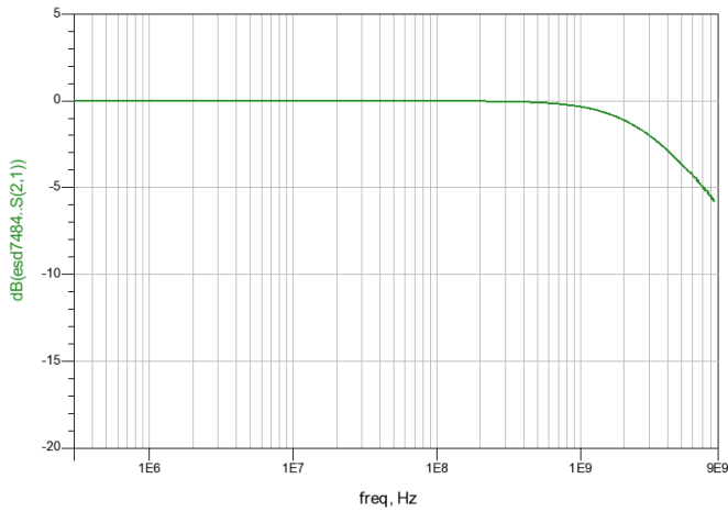
Figure 3. S21 Plot
