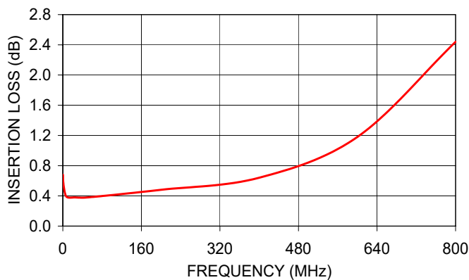
INSERTION LOSS
