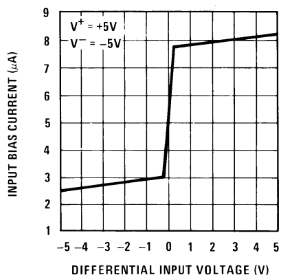
Input Characteristics
