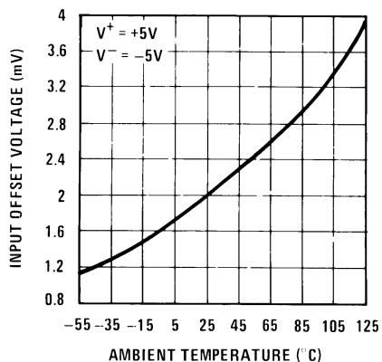
Offset Voltage
