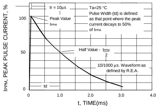
FIG.3 - PULSE WAVEFORM
