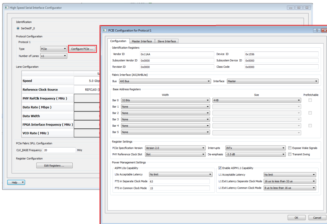
Figure 4-6. High-Speed Serial Configurator with PCIe Implementation Options
