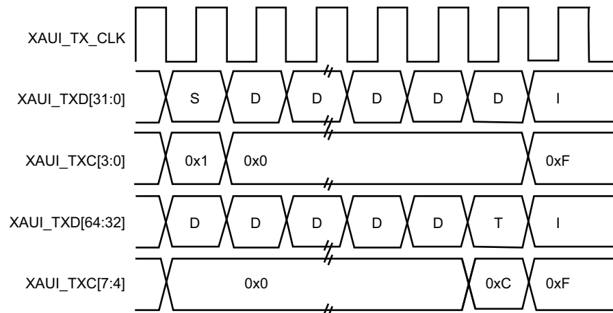
Figure 5-12. Transmit XGMII Interface Timing Diagram
