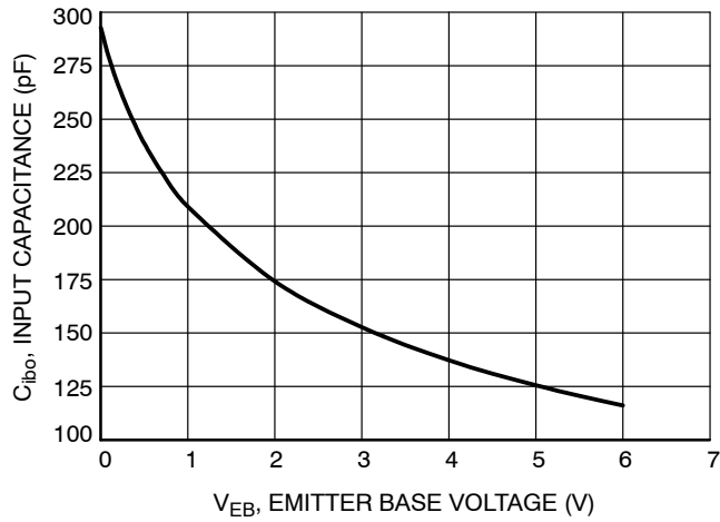
Figure 21. Input Capacitance
