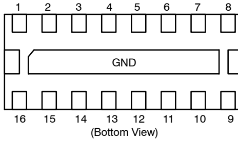
Figure 3. Pin Diagram
